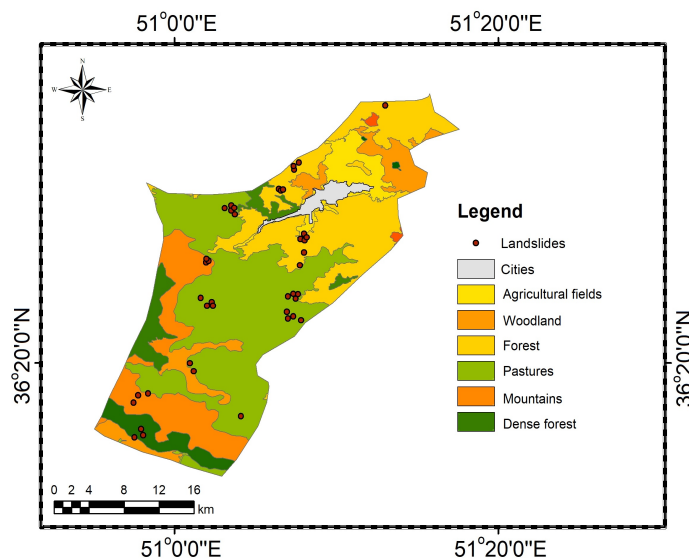
Fig. 6 The land-use map for studied area
