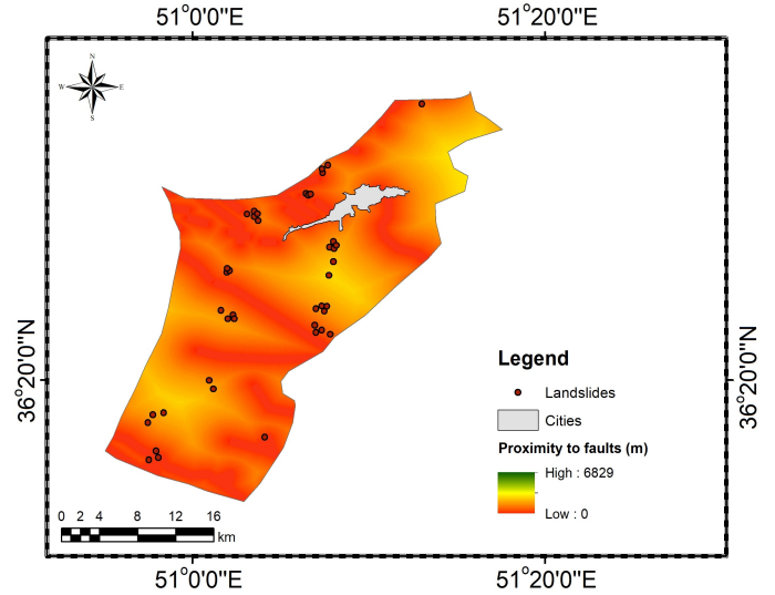
Fig. 7 Distance to the faults in studied area
