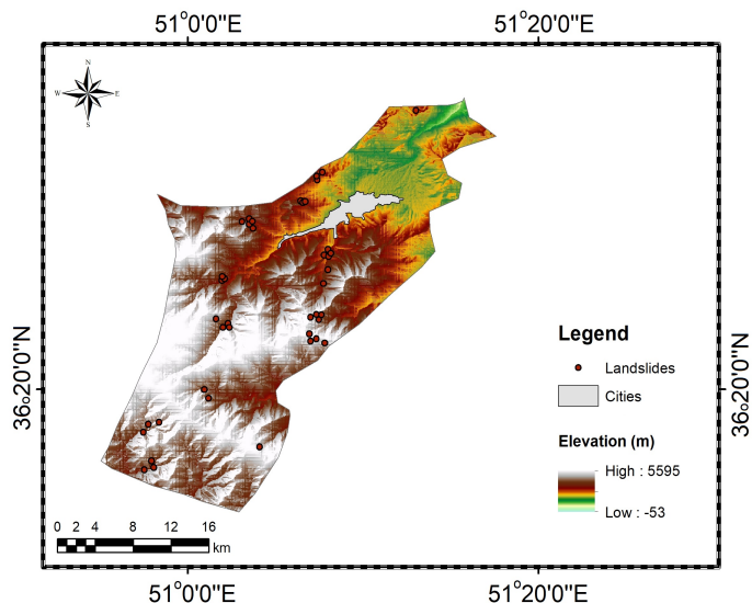
Fig. 12 Elevation variations in studied area
