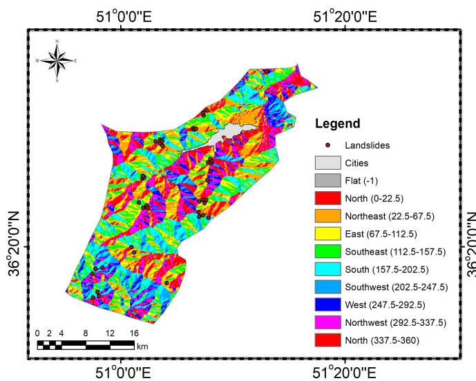
Fig. 5 Slope aspect variation in studied area
