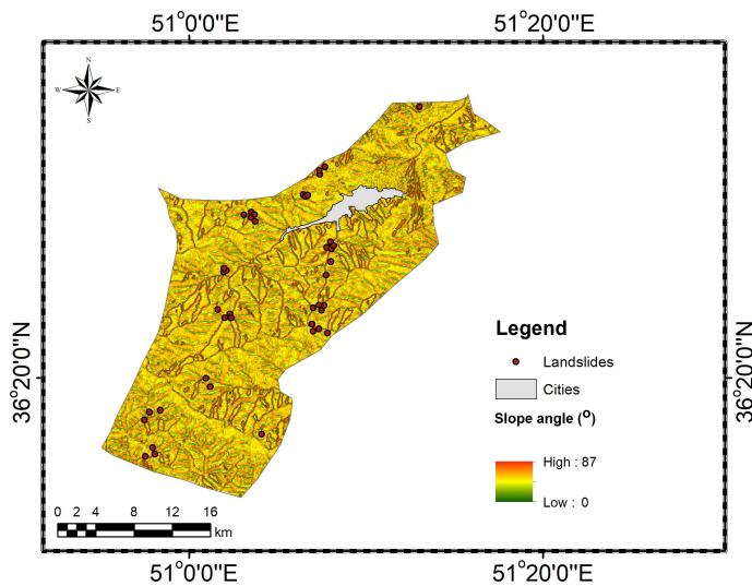
Fig. 4 Slope angle variation in studied area
