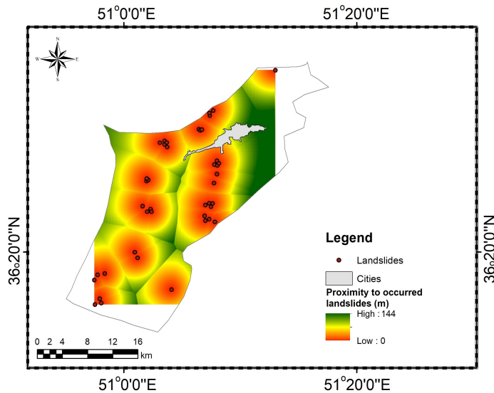
Fig. 10 Distance to the occurred landslides in studied area
