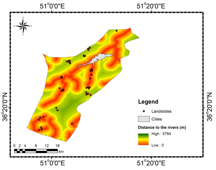
Fig. 8 Distance to the rivers in studied area
