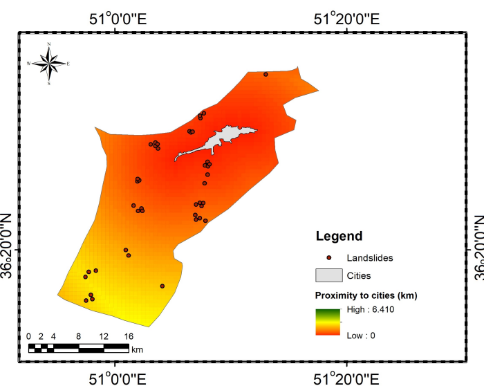
Fig. 9 Distance to the cities in studied area
